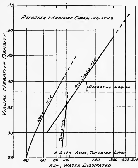
FIG. 3. Exposure characteristics of light-sources for release type Western Electric Recorder. Dupont 222, special negative developer, gamma 0.28; (a) air-cooled H3X arc; (b) H3X arc; and (c) 9.5-v, 9-ampere coiled-filament tungsten lamp.
